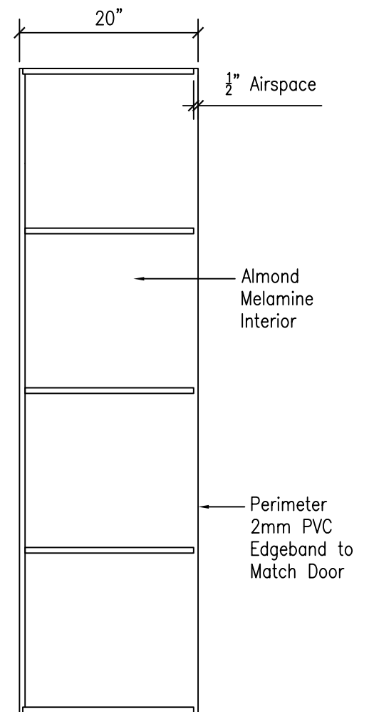
SECTION
