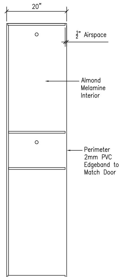
SECTION
